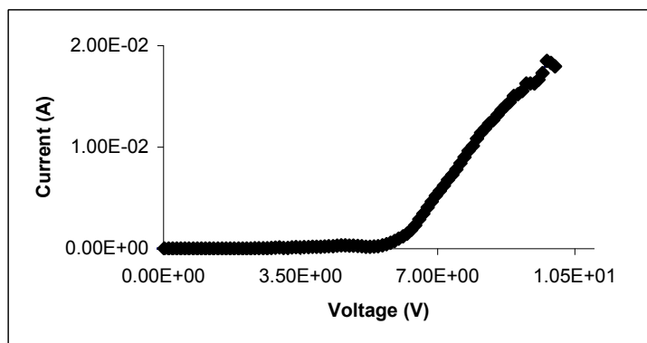
Figure 1 Current-voltage characteristic of the thin film
